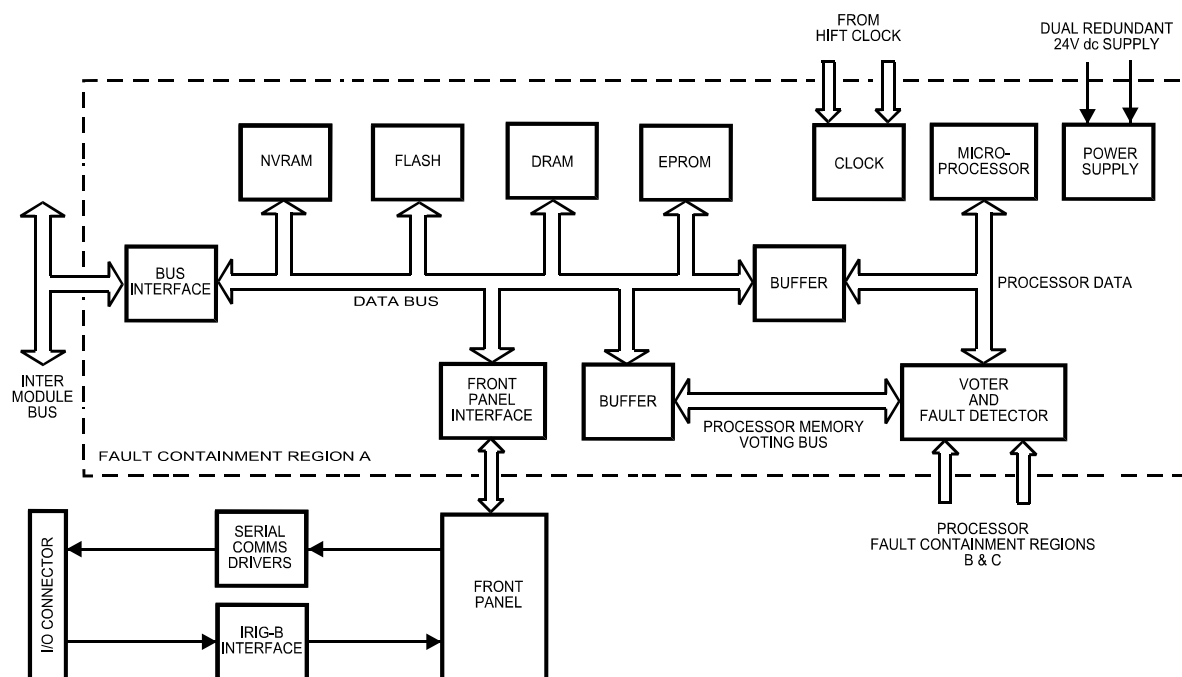
Figure 1 Module Architecture
